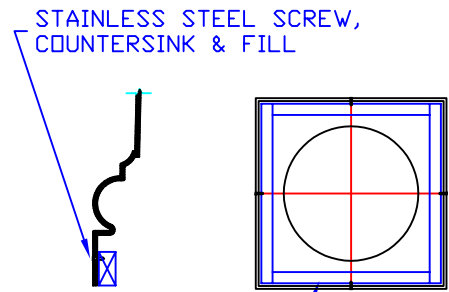
BLOCKING AS REQUIRED BLOCKING DETAIL, BASE
