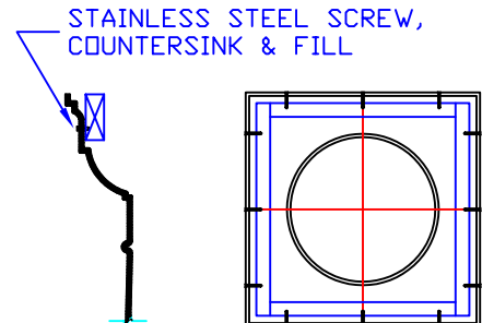
BLOCKING AS REQUIRED BLOCKING DETAIL, CAPITAL
