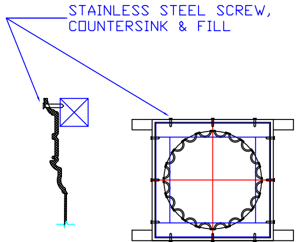
BLOCKING AS REQUIRED BLOCKING DETAIL, CAPITAL
