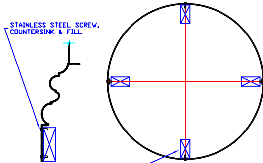
BLOCKING AS REQUIRED BLOCKING DETAIL, BASE
