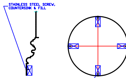
BLOCKING DETAIL, BASE
