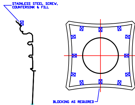
BLOCKING DETAIL, CAPITAL
